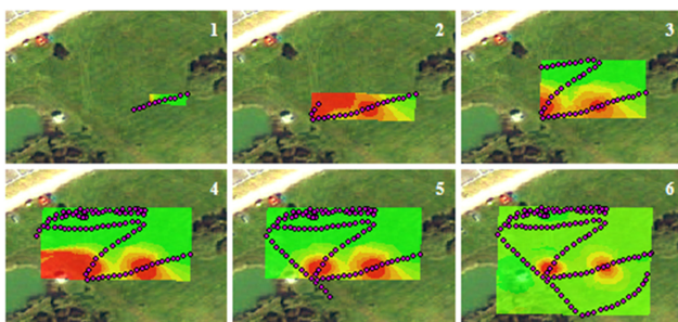
Figure 6. Growing Interpolation Result for Radiation Source Identification.
